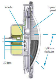
Drawing shows lens and reflector design which combine to provide superior light beam distribution.
